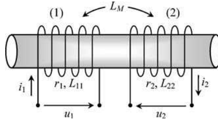
Figure 7.35 Two-windings transformer
