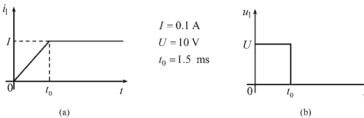
Figure P10.2 (a) Current i_1 against time (ramp shape). (b) Voltage u_1 against time (rectangular pulse)
