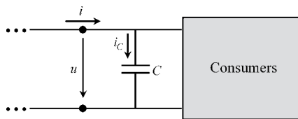
Figure P1.3 A capacitor is placed at the far end of the line for power factor compensation purposes
