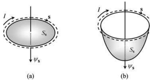
Figure 4.15 The magnetic flux linkage \psi in (a) and (b) is the same. The particular shape of the open surfaces bounded by the path \mathbf{s} is irrelevant for the evaluation of \psi
