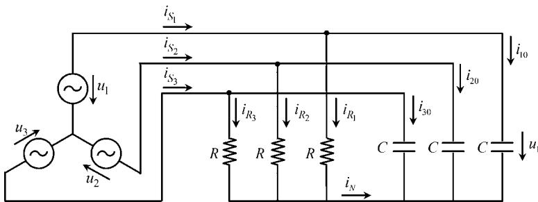
Figure P15.4 Equivalent circuit for the configuration shown in Figure P15.3
