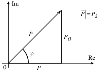
Figure 7.10 Triangle representation of powers
